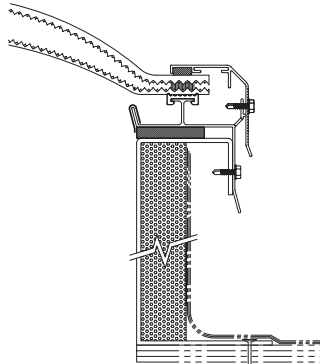
ALIB - Aluminum framed skylight with UL/FM Compliant Polyvinyl Chloride (PVC) thermal barrier break and insulated base. Available as self flashing only. (Shown with optional curb seal tape)
