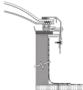
ALIT - AAMA Compliant thermally broken aluminum framed skylight with insulated base. Available as self flashing only. (Shown with optional curb seal tape and aluminum welded double wall)
