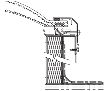
ALT - AAMA Compliant thermally broken aluminum framed skylight. Available as curb mounted or self flashing. (Self flashing model shown)
