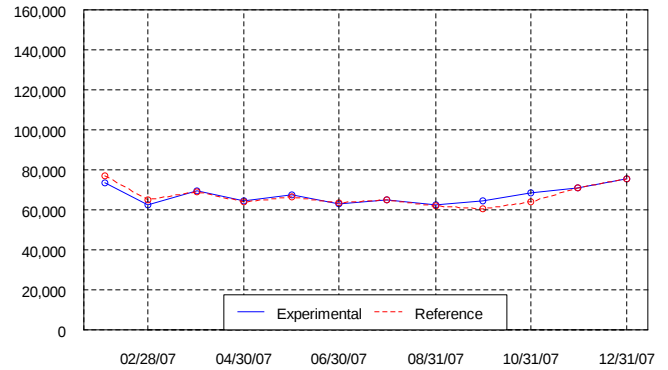
McKinney Sales Floor & Perimeter Lighting kWh/month
