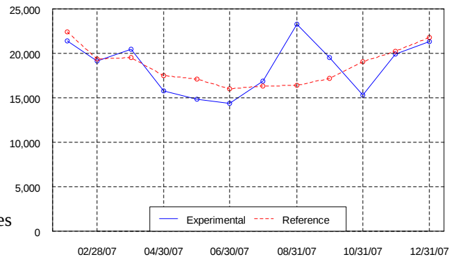
McKinney Parking Lot Lighting kWh/month
