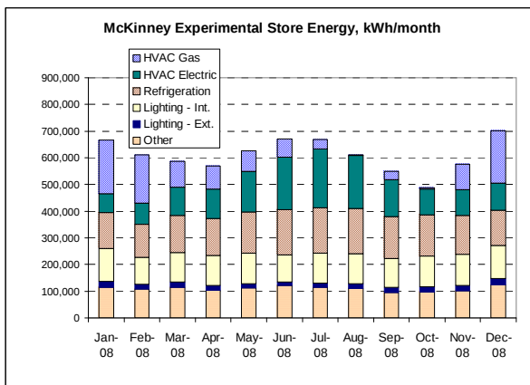
Figure 11 – Experimental Store End-Use Energy
