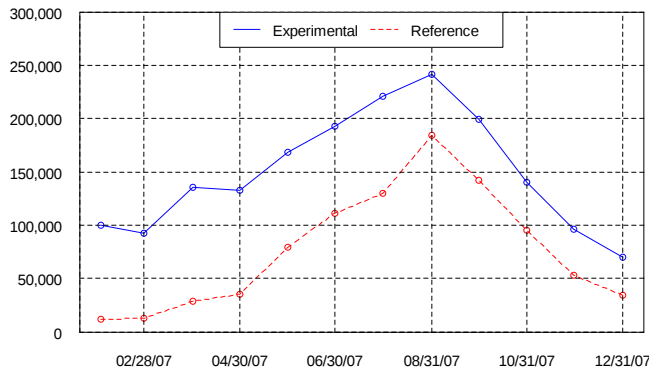
McKinney HVAC Electric kWh/month
