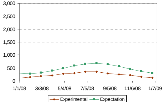
PV Array 3 Production, kWh/month TLE Roof Modules
