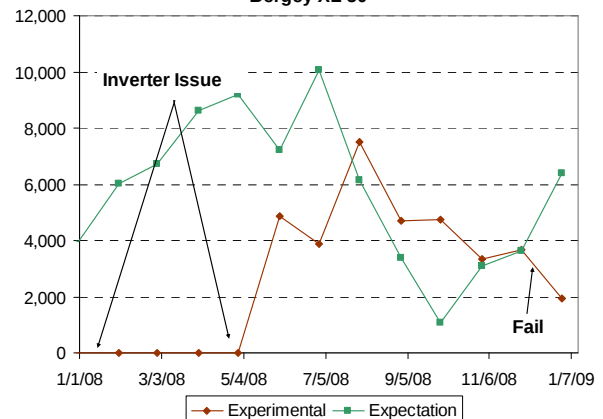
50-kW Wind Turbine Production, kWh/month Bergey XL 50
