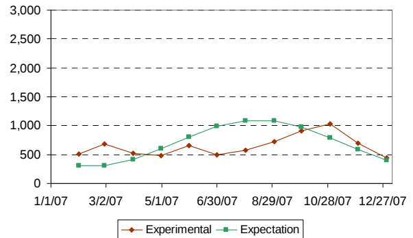
PV Array 4 Production, kWh/month SkyView Modules, Garden Center Roof
