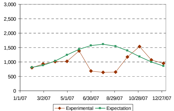
PV Array 4 Production, kWh/month SkyView Modules, Garden Center Roof
