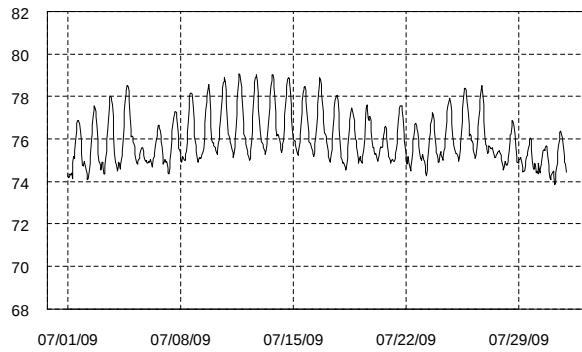
Experimental Store TH3-13ft Level, F
