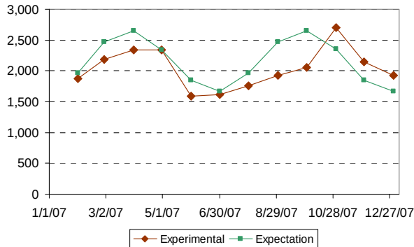
PV Array 5 Production, kWh/month Clerestory Crystalline and Asi-Thru Thin-Film
