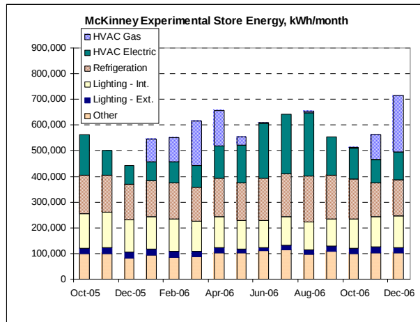
Figure 5 — Experimental Store End-Use Energy
