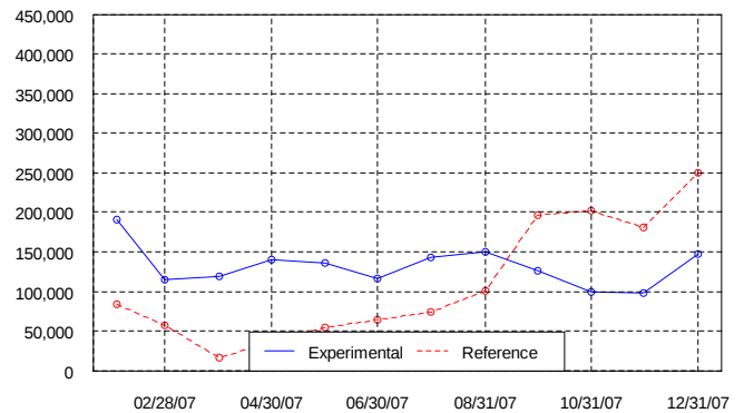
McKinney Sales Floor Total HVAC kWh/month
