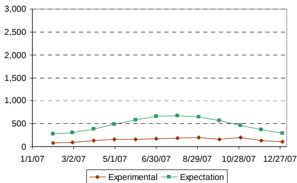
PV Array 3 Production, kWh/month TLE Roof Modules
