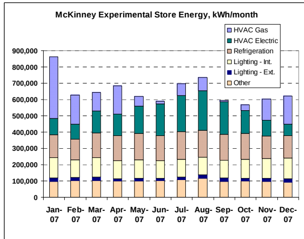
Figure 8 — Experimental Store End-Use Energy
