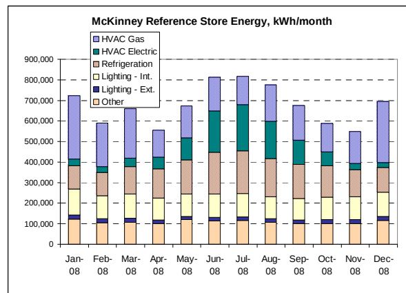
Figure 12 – Reference Store End-Use Energy
