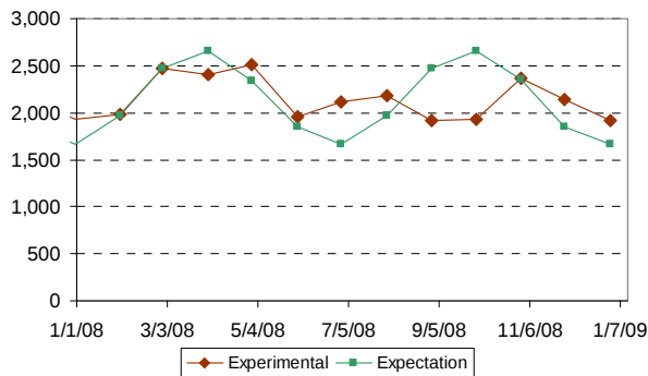
PV Array 5 Production, kWh/month Clerestory Crystalline and Asi-Thru Thin-Film
