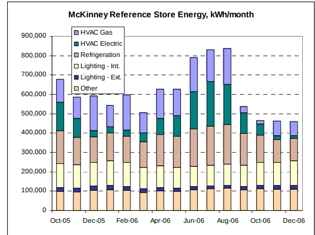
Figure 6 — Reference Store End-Use Energy
