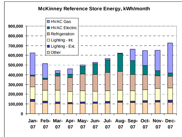
Figure 9 — Reference Store End-Use Energy
