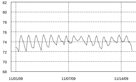
Experimental Store TH3-5ft Level, F
