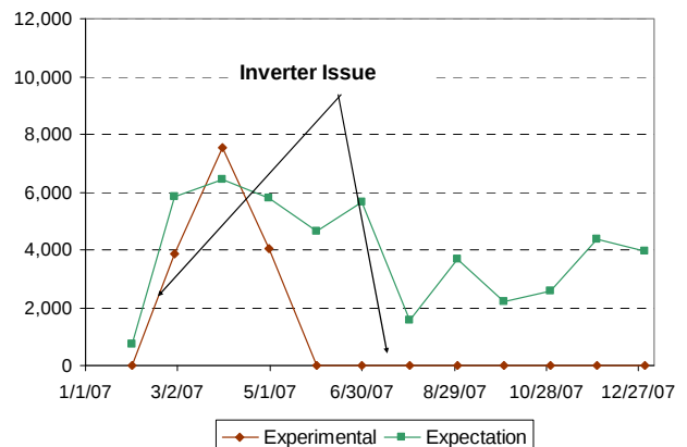
50-kW Wind Turbine Production, kWh/month Bergey XL 50
