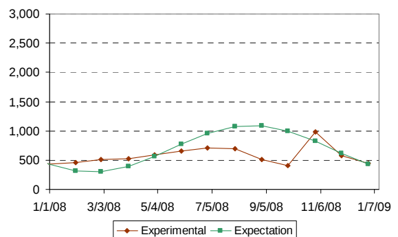
PV Array 4 Production, kWh/month SkyView Modules, Garden Center Roof
