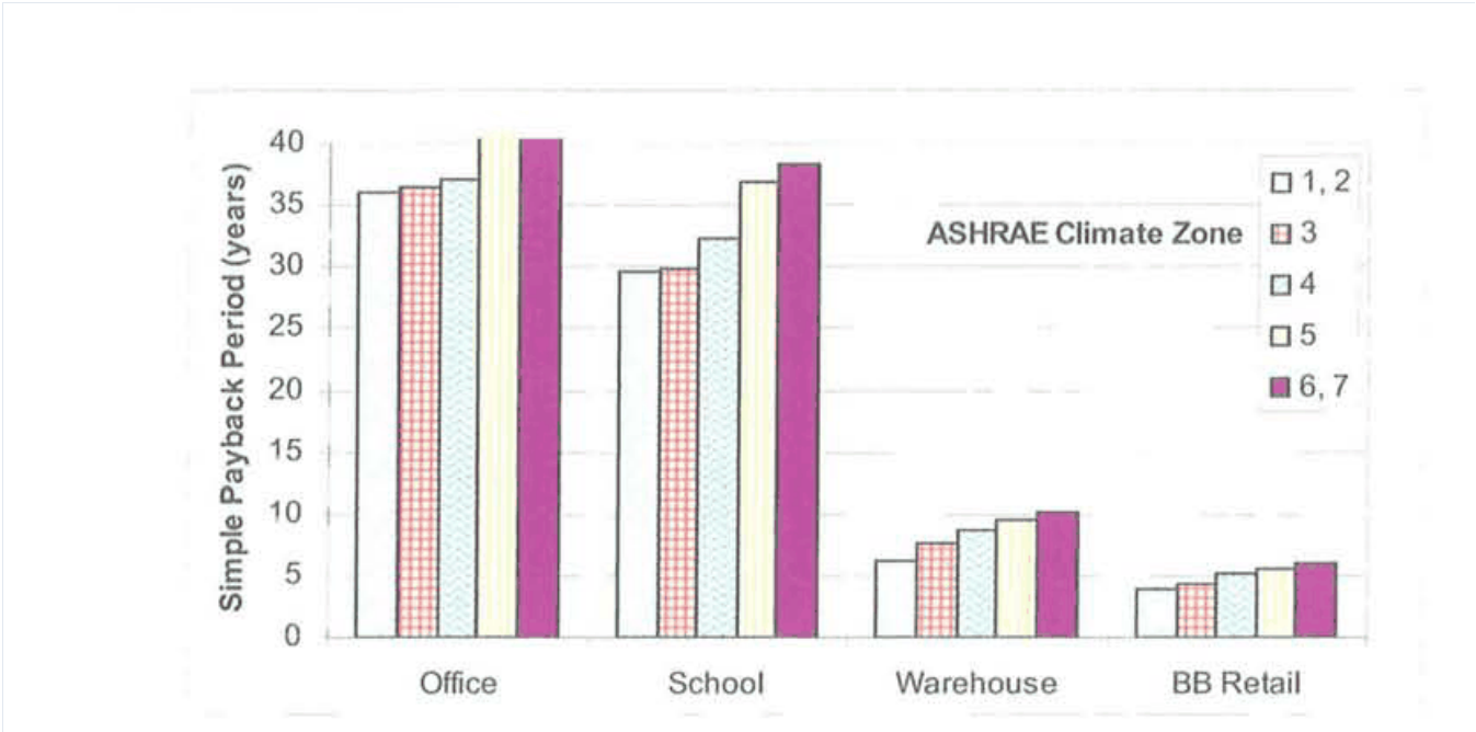
Figure 7-1: Simple Payback Resulting From Energy Savings, by Climate Zone and Building Type
