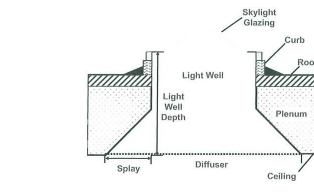
Figure 3-3: Typical Skylight System
