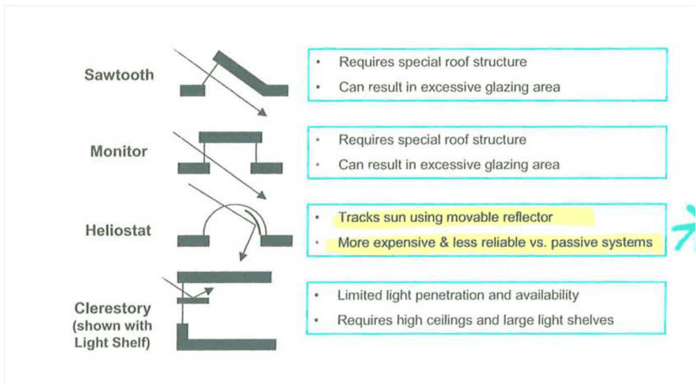
Figure 3-2: Alternative Toplighting Methods
