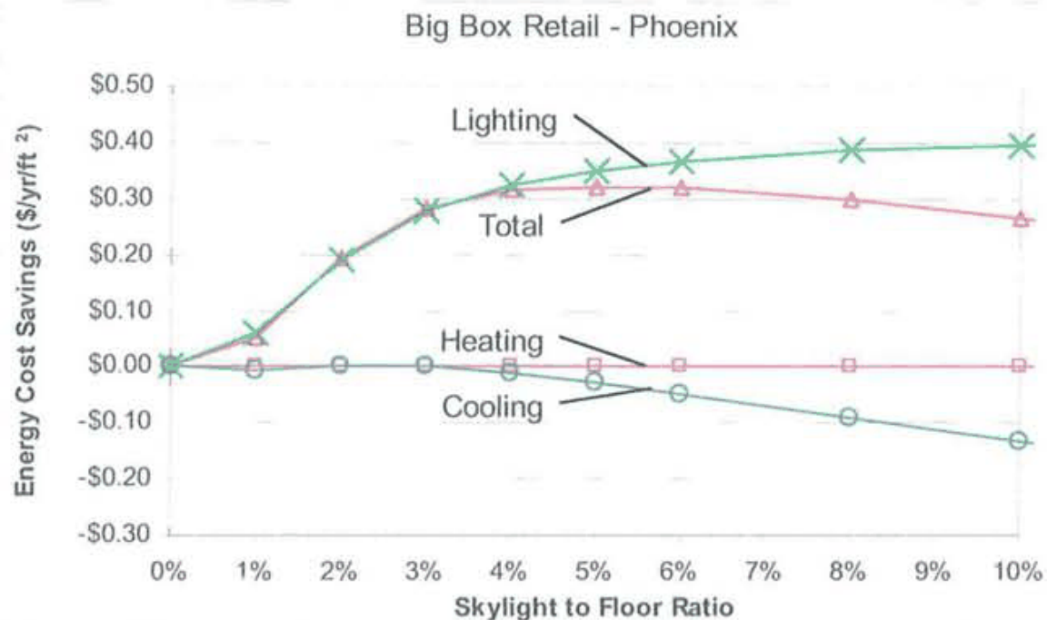
Figure 5-5: Annual Energy Cost Savings by End Use (lighting, cooling, heating) as a Function of SFR, Phoenix
