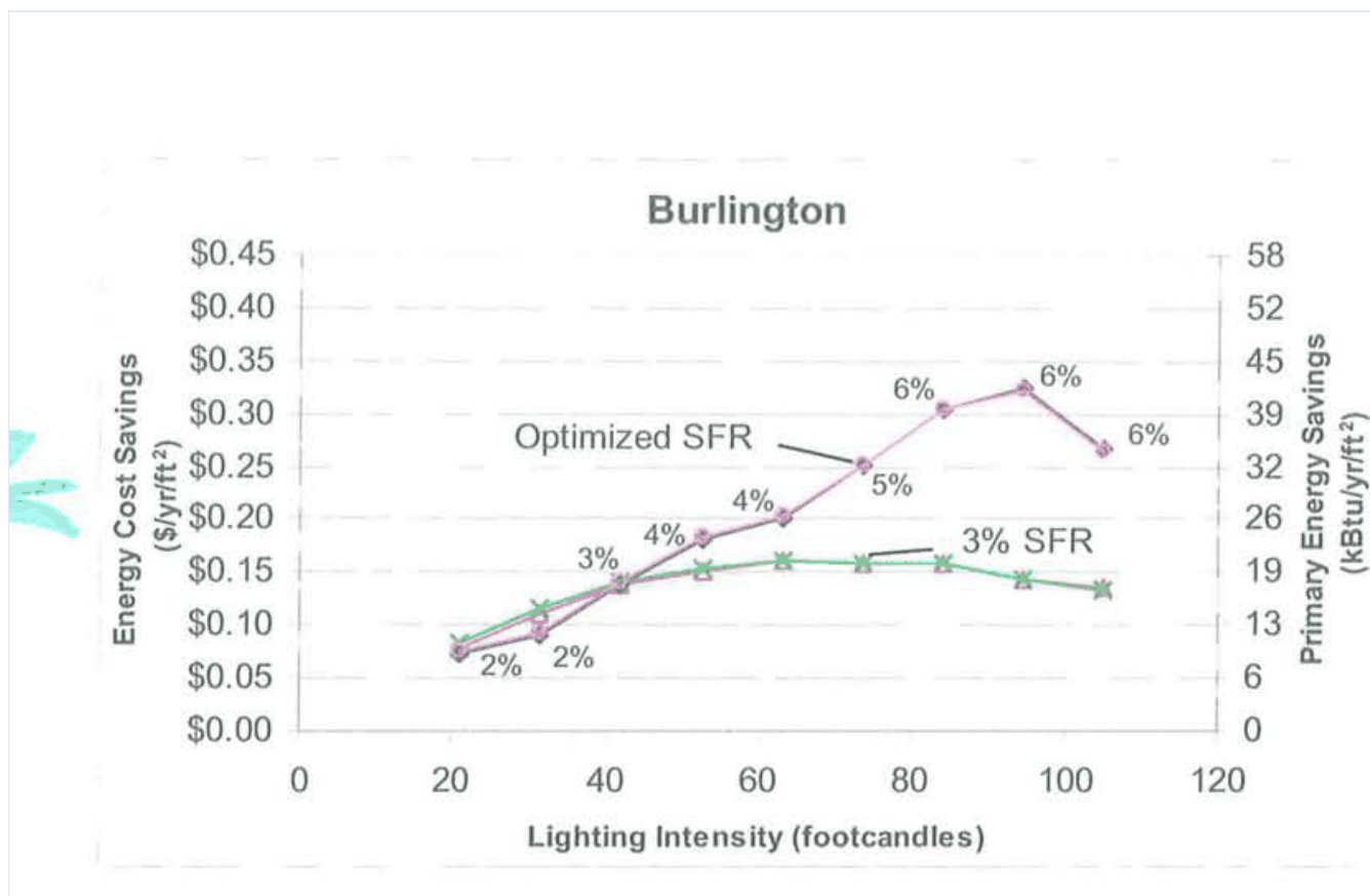
Figure 4-3: Energy Cost Savings as a Function of Required Lighting Intensity / Lighting Power Density, Big Box Retail, Burlington
