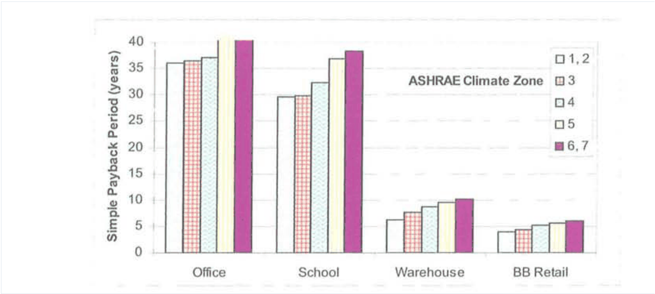
Figure 1-1: Simple Payback Resulting From Energy Savings, by Climate Zone and Building Type
