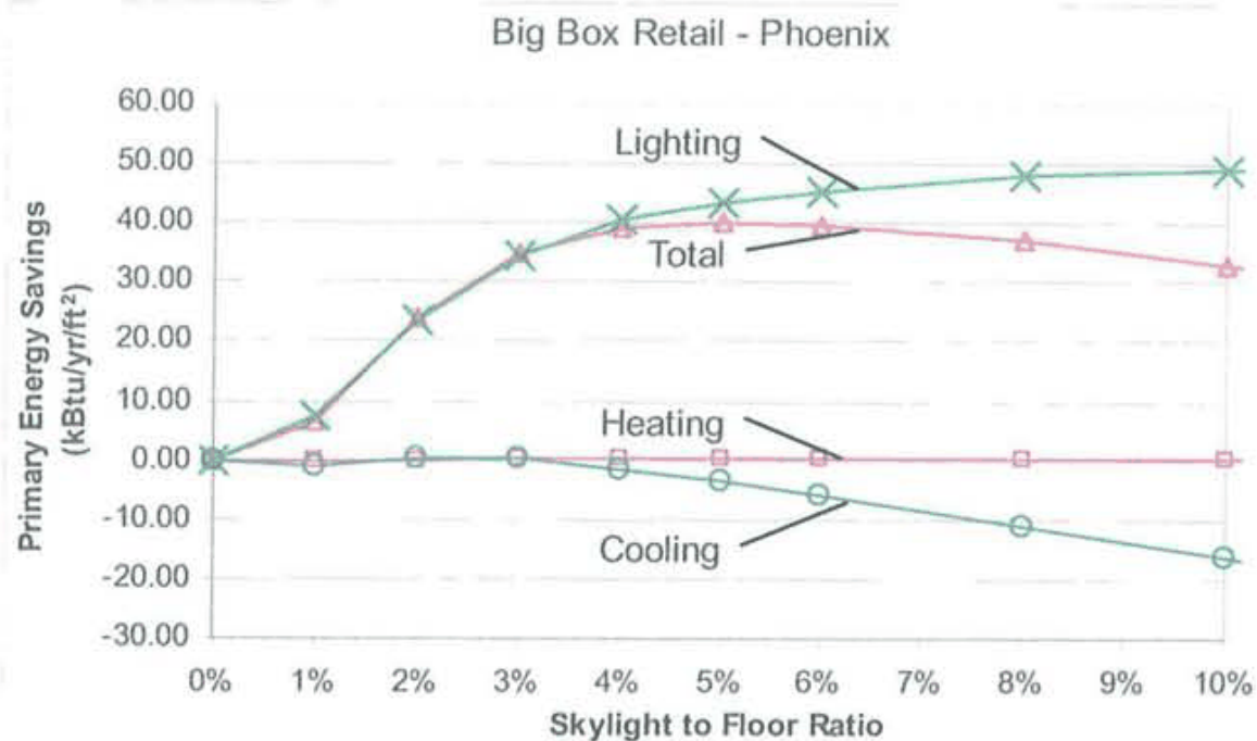
Figure 5-4: Annual Primary Energy Savings by End Use (lighting, cooling, heating) as a Function of SFR, Phoenix
