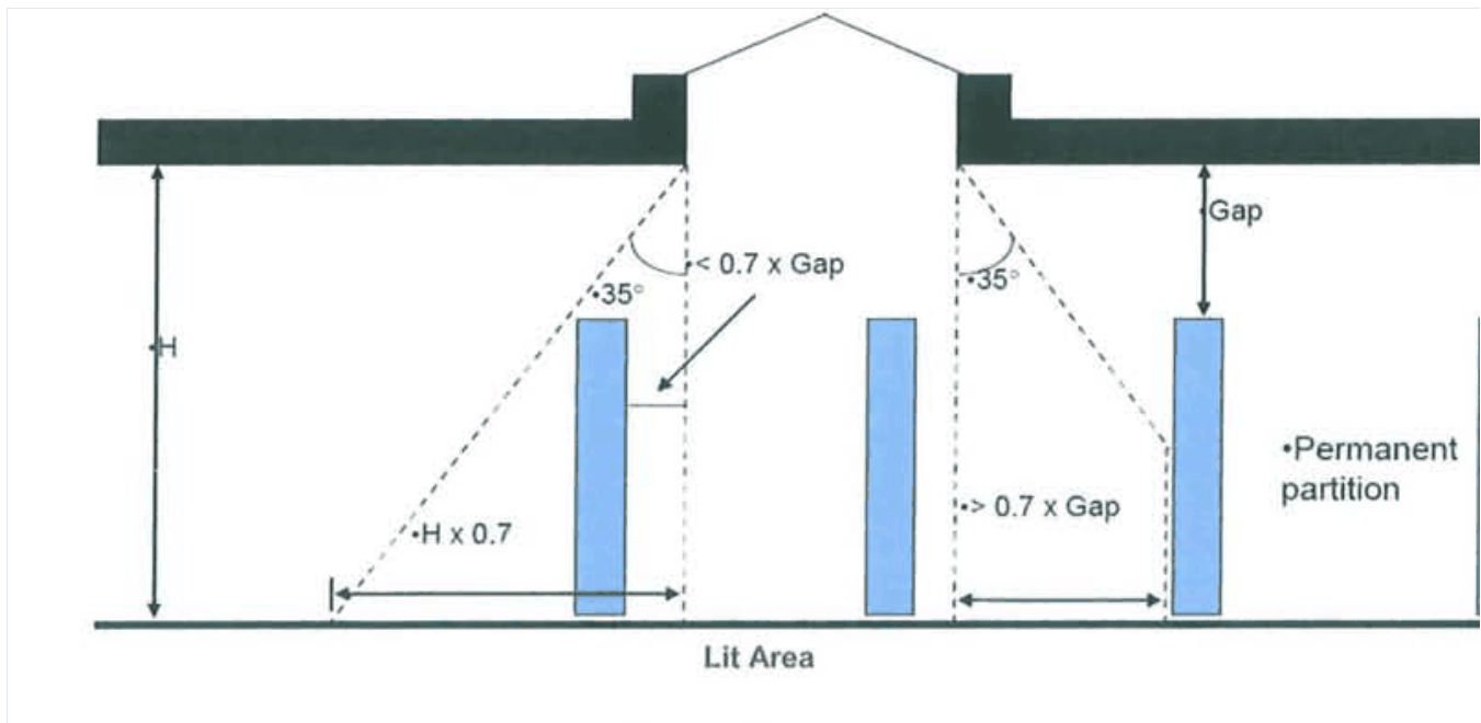
Figure 4-1: Skylight Spacing Criteria (PG&E 2006)
