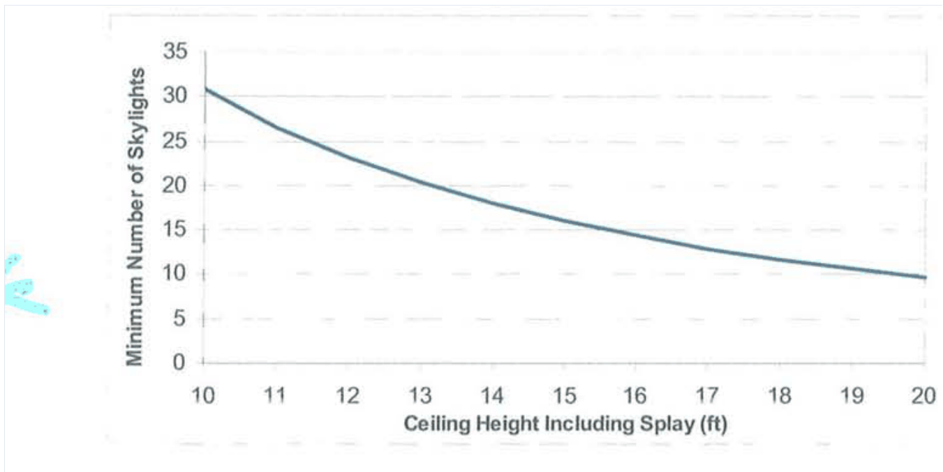
Figure 4-2: Number of Skylights Required for a 10,000 ft 2 Area Versus Ceiling Height
