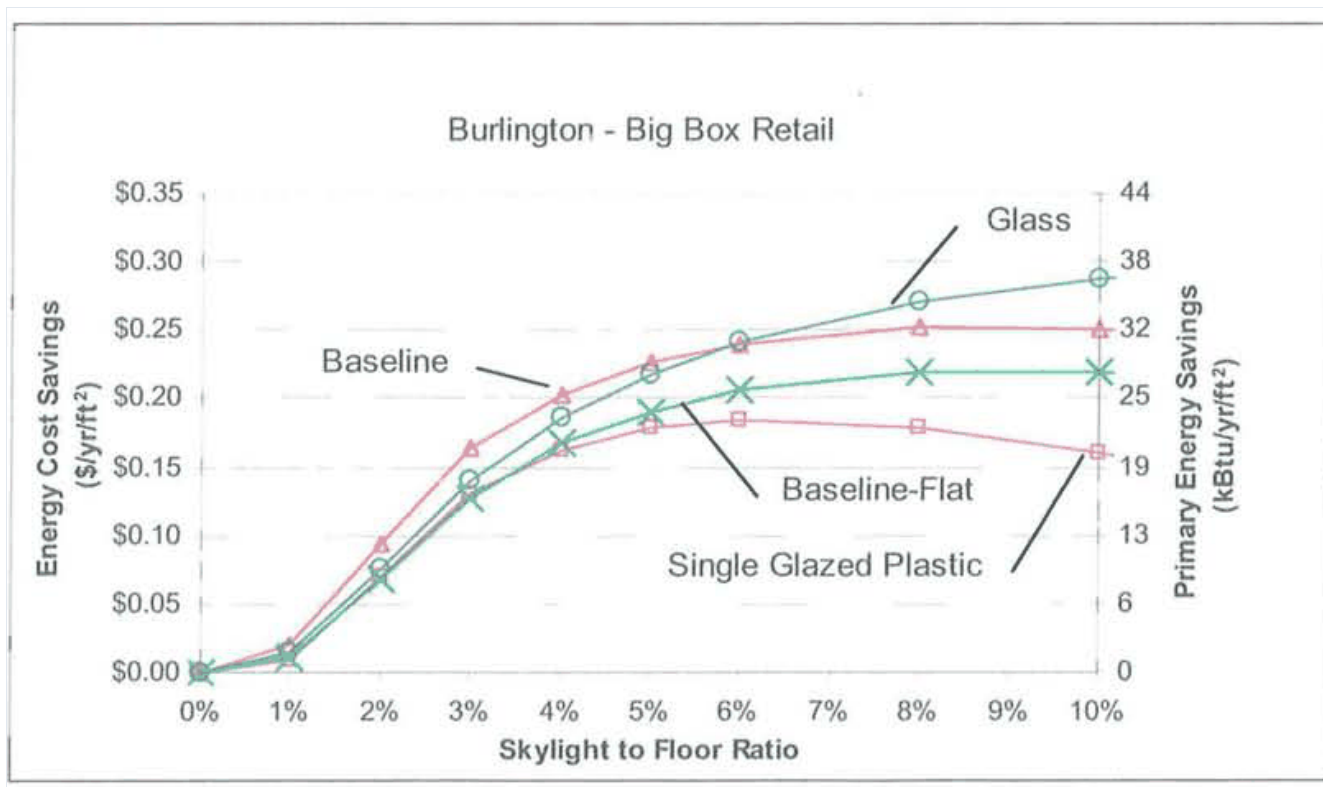
Figure 4-9: Effect of Skylight Type, Big Box Retail, Burlington
