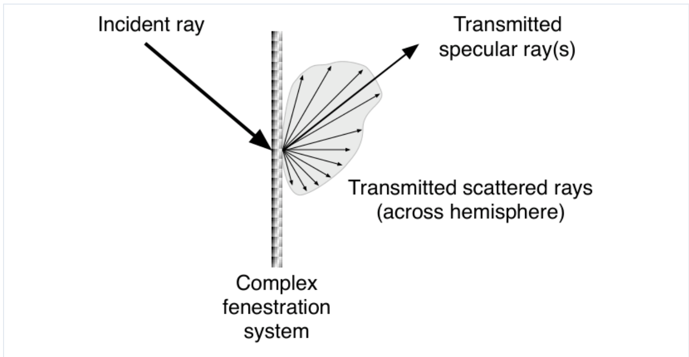
Figure 1: Schematic showing the distribution in transmitted light from a complex fenestration system
