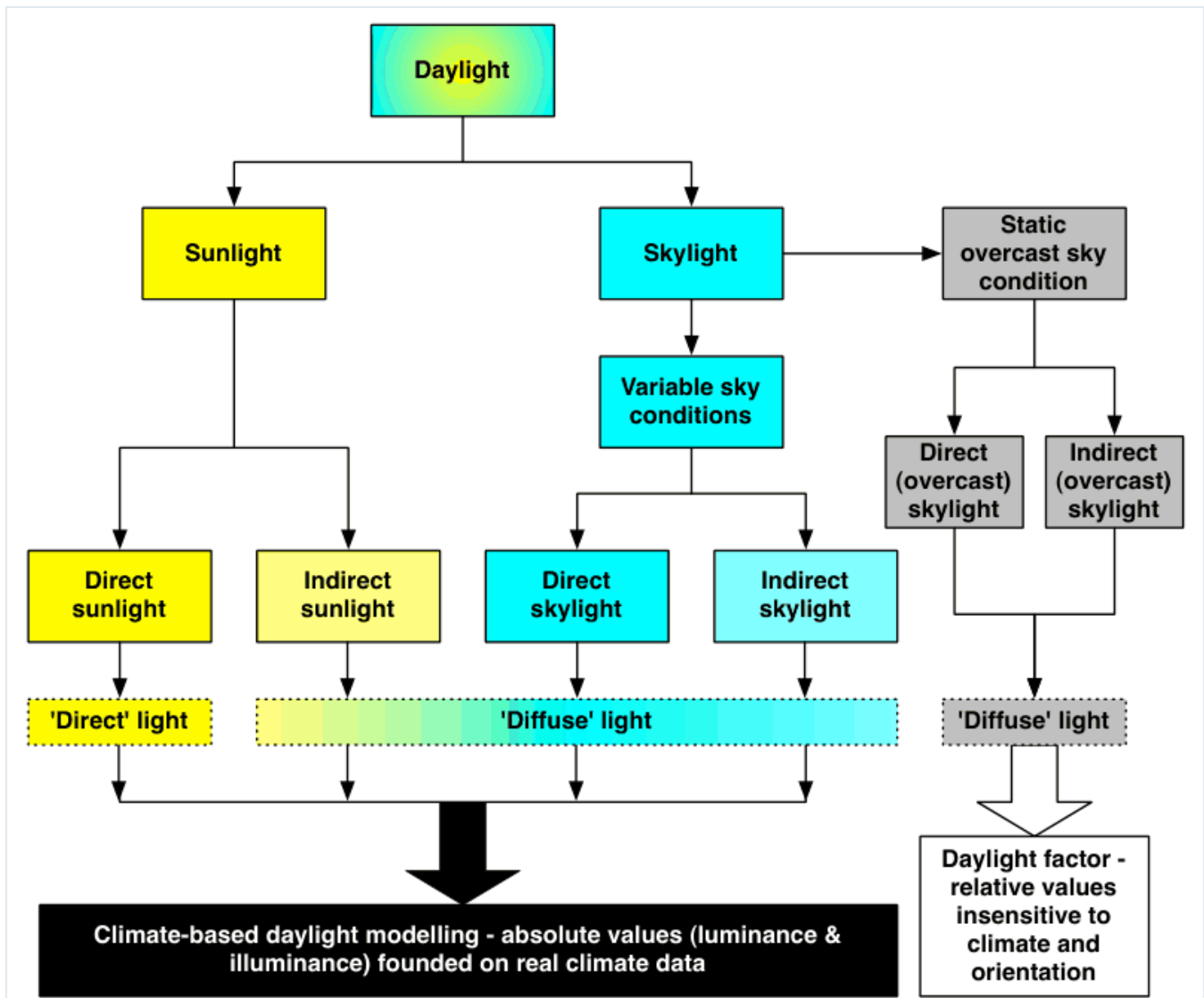
Figure 3: The components of daylight and their relation to the daylight factor and climate-based modelling approaches
