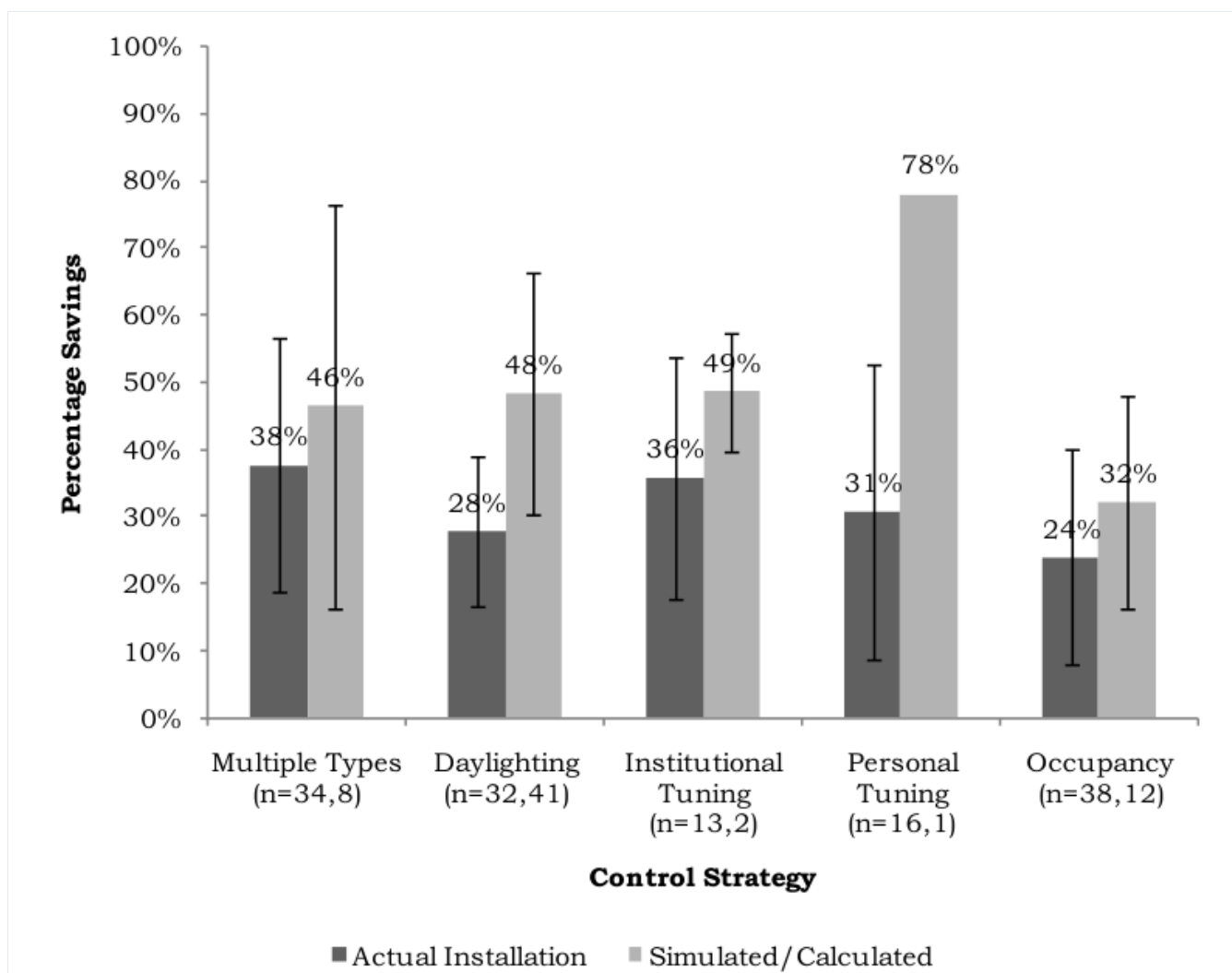
Fig. 5. Comparison of energy savings for actual installations and simulated or calculated installations.
