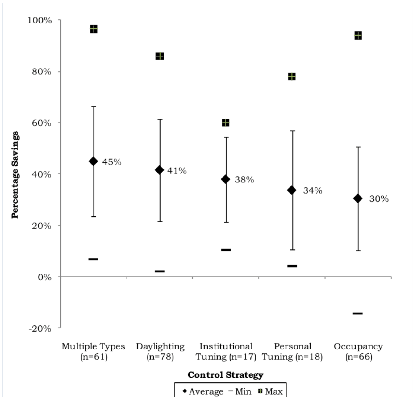
Fig. 2. Average savings (%) by control type – unfiltered; error bar shown represents one standard deviation.
