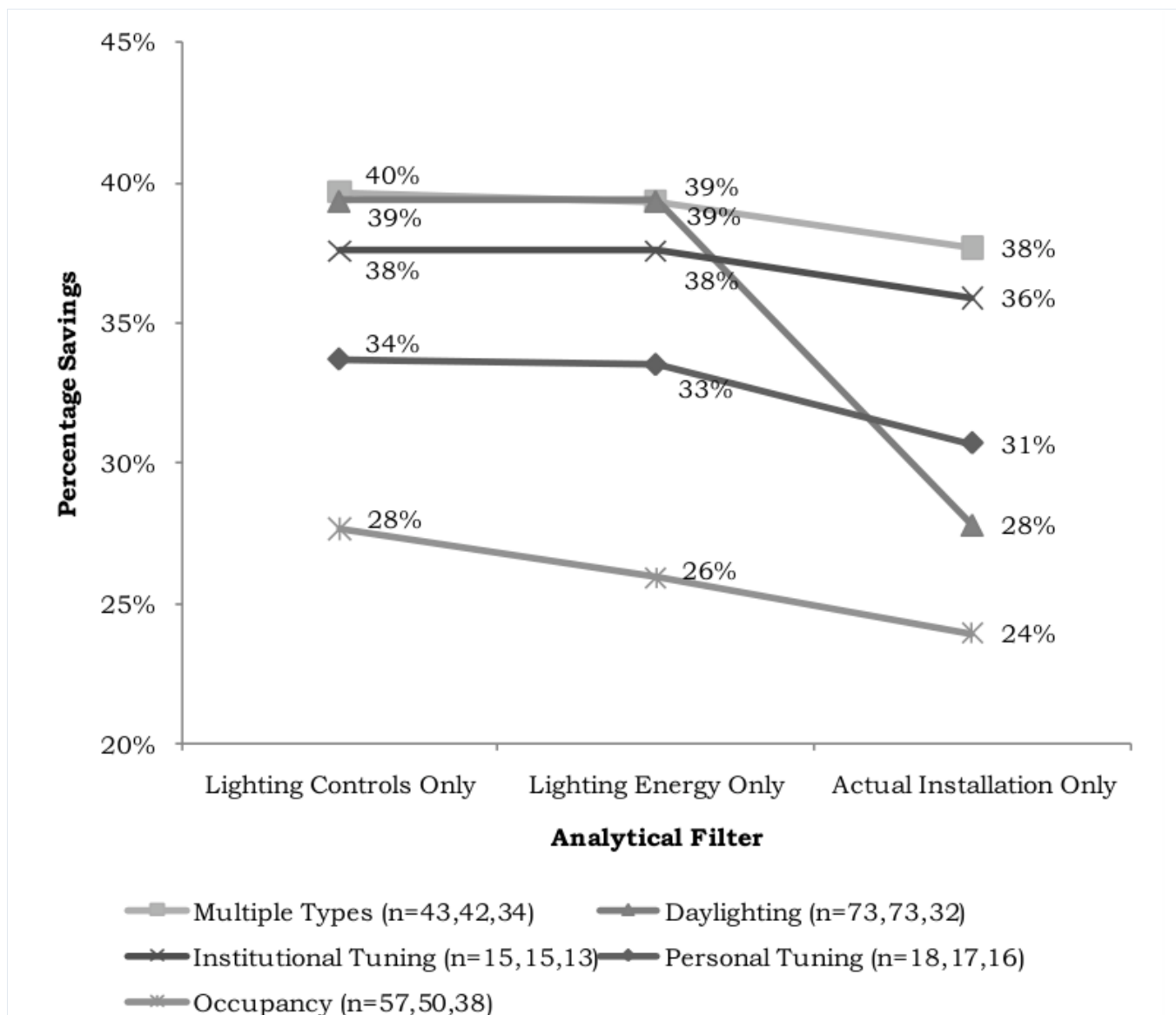
Fig. 8. Comparison of energy savings from first filter to final filter.
