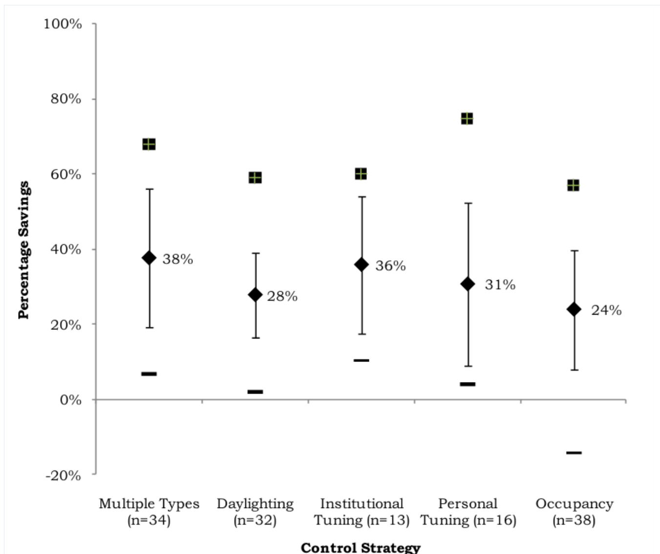
Fig. 6. Energy savings for lighting controls and lighting energy in actual installations – final filter; symbols as shown in Fig. 2.
