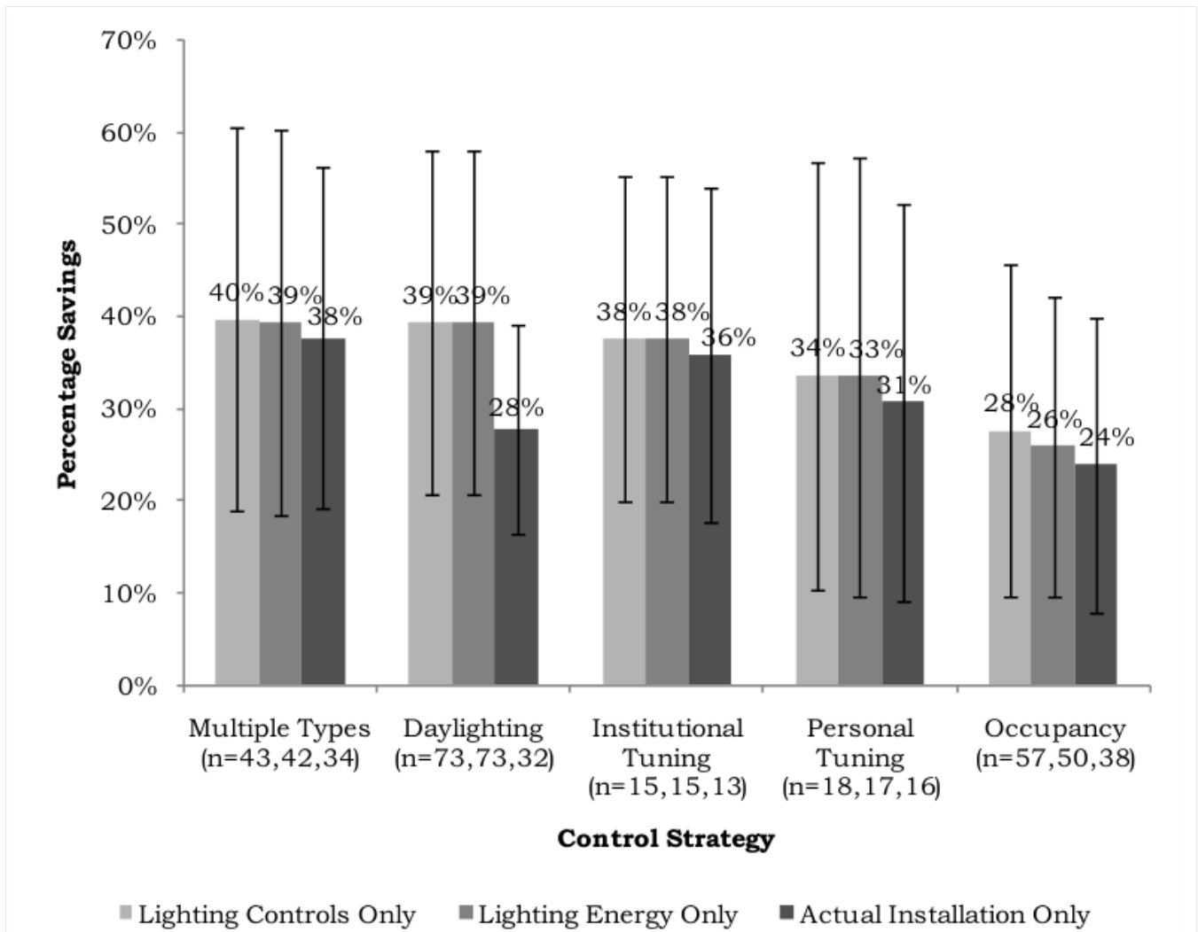
Fig. 7. Comparison of energy savings from first filter to final filter. (Note that we do not show the overall unfiltered results here; because it includes savings from non-controls-related measures, it is not relevant to the final analysis).
