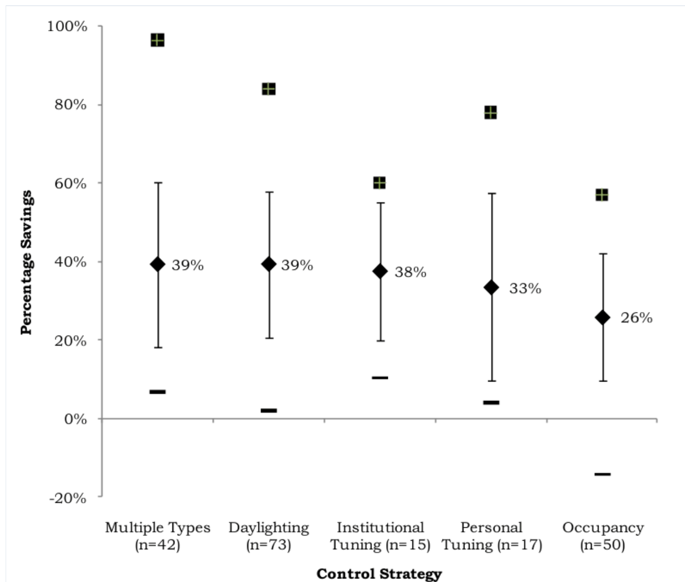
Fig. 4. Energy savings for lighting controls and lighting energy only – second filter; symbols as shown in Fig. 2.
