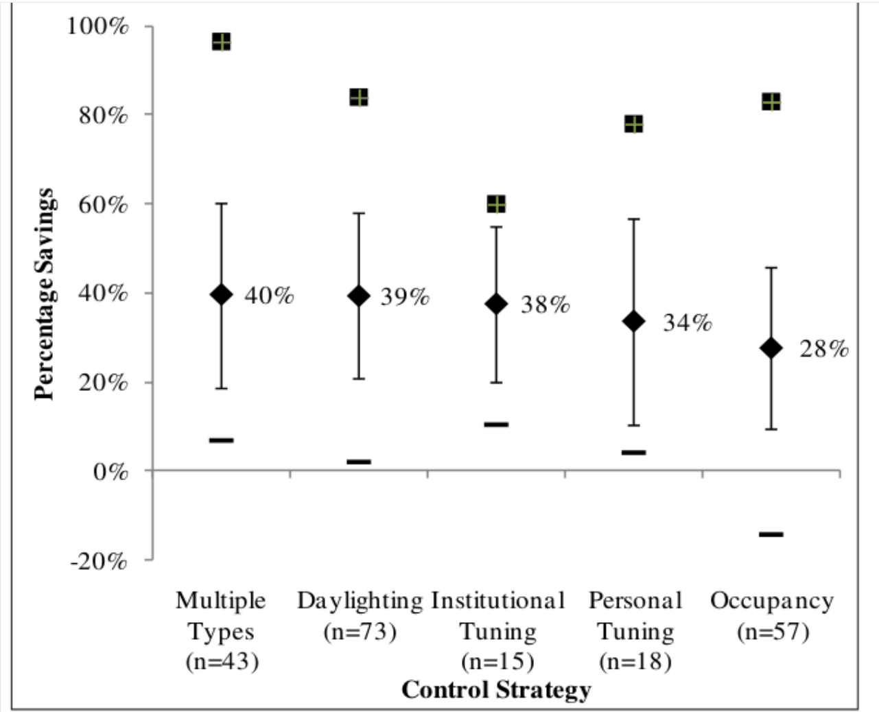
Figure 2. Energy Savings for Lighting Controls Only. Symbols as shown in Figure 1.
