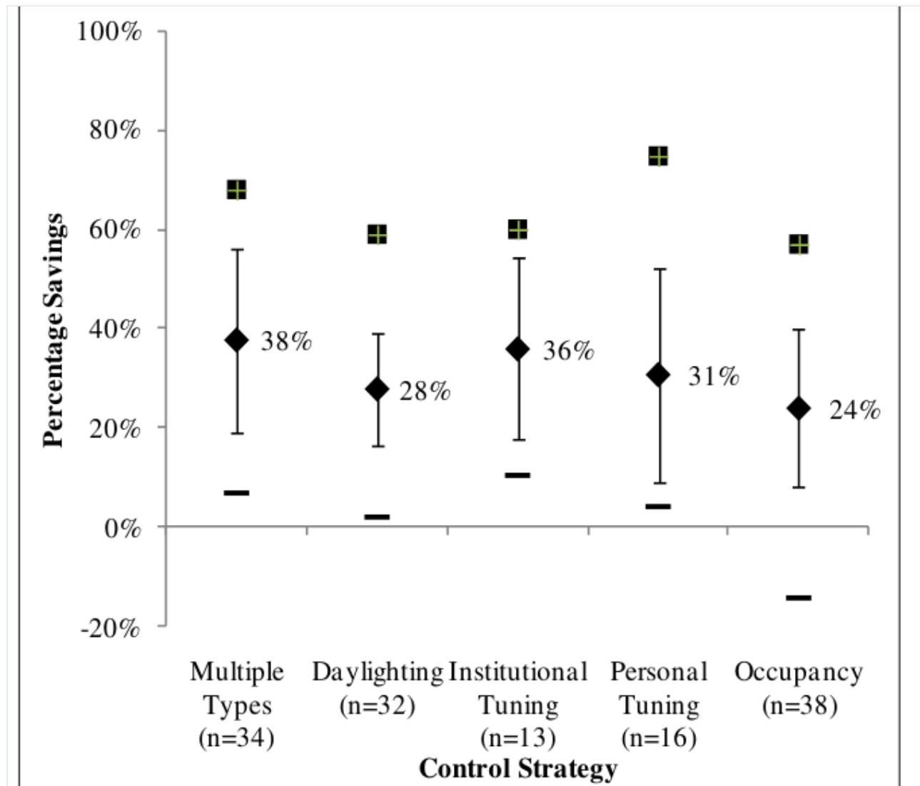
Figure 4. Energy Savings for Lighting Controls and Lighting Energy in Actual Installations. Symbols as shown in Figure 1.
