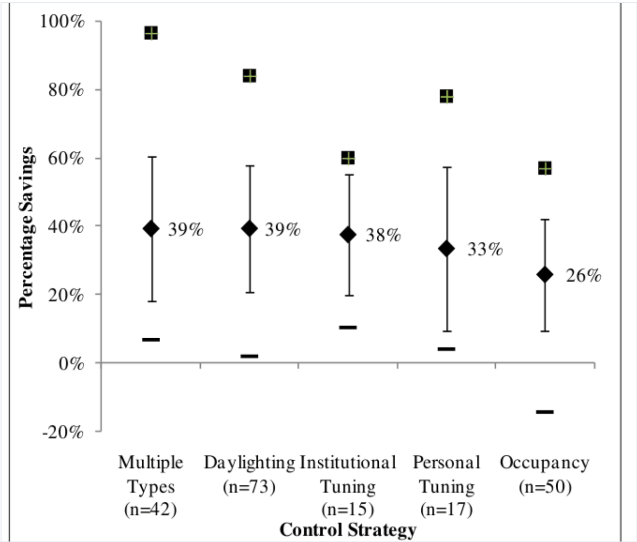
Figure 3. Energy Savings for Lighting Controls and Lighting Energy Only. Symbols as shown in Figure 1.
