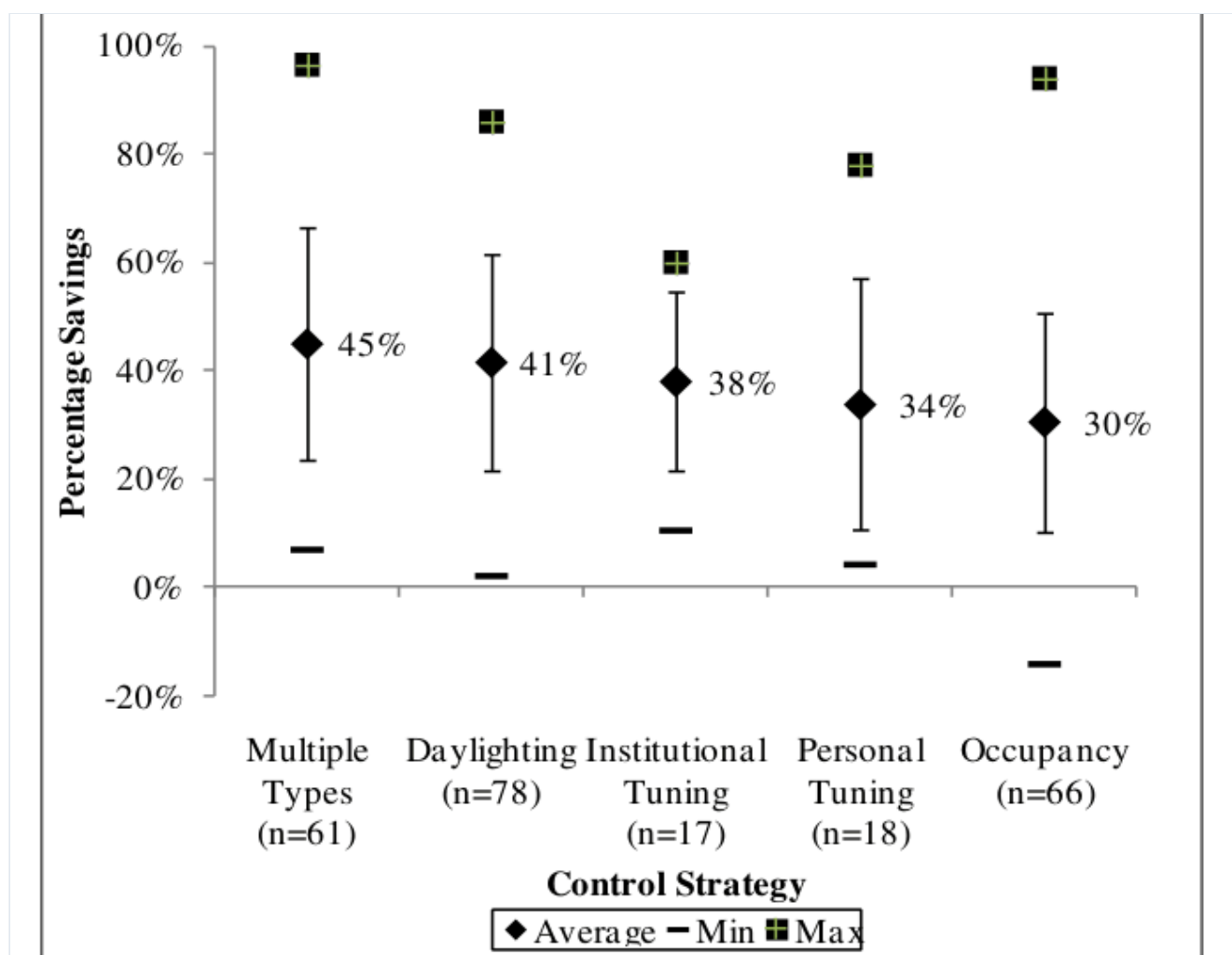
Figure 1. Average Energy Savings (%) By Control Strategy. Error bar shown represents one standard deviation.
