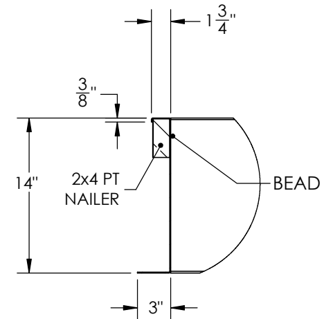
DETAIL B SCALE 1 : 12
