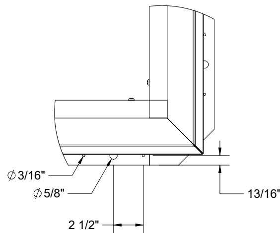
DETAIL C SCALE 1 : 8
