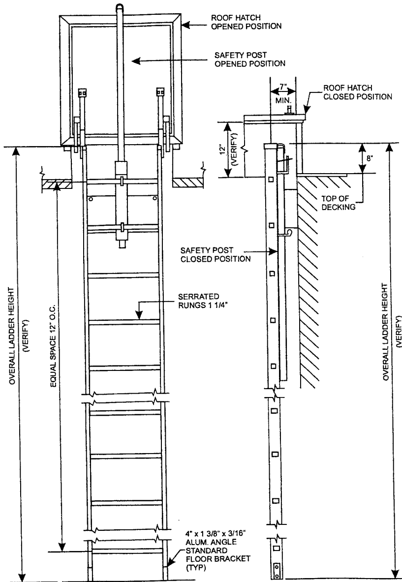
SIDE ELEVATION
