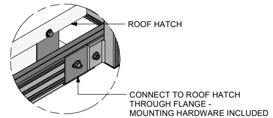
DETAIL C
