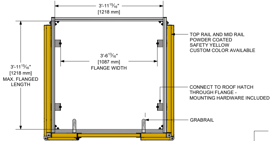
TOP VIEW
