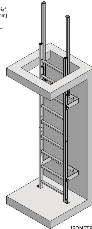
ISOMETRIC VIEW
