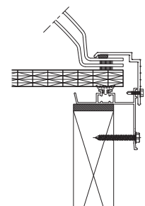
Triple Glazed with 16mm Polycarbonate Multi-wall
