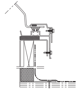
Si: Self-Flashing base with 1" insulation - available with or without Wood Nailer (WN)
