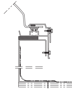
SF: Self-Flashing Base constructed of 0.063" to 0.125" aluminum (non-structural curbs).
