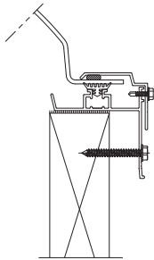
CM: Curb mounted skylight requires use of sealant or customer supplied foam tape to seal to curb
