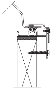
CT: Curb mounted skylight with EPDM foam tape to seal against curb
