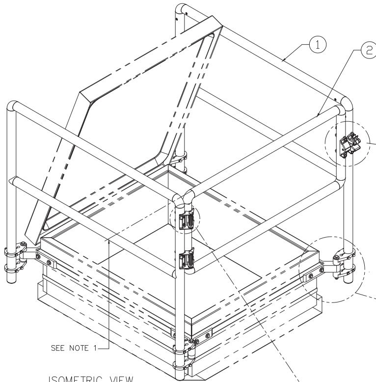
ISOMETRIC VIEW
