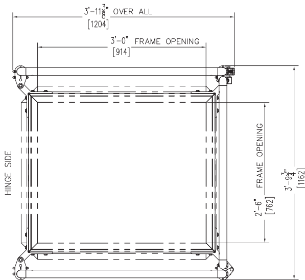
PLAN VIEW SHOWN WITHOUT COVER
